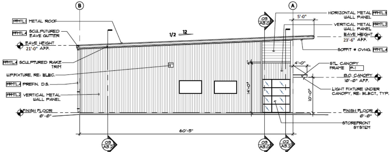
Typical Side Elevation Over 20' of clearance
